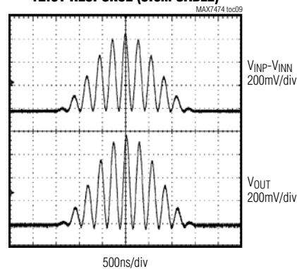
12.5T RESPONSE (0.5m CABLE)
