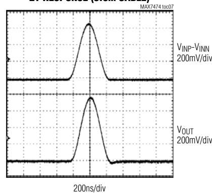
2T RESPONSE (0.5m CABLE)
