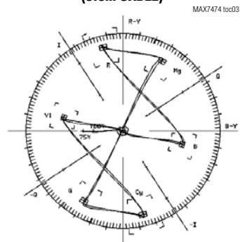
75% COLOR BAR VECTOR DIAGRAM (0.5m CABLE)
