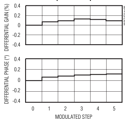
DIFFERENTIAL GAIN AND PHASE (300m CABLE)
