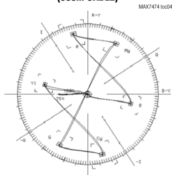
75% COLOR BAR VECTOR DIAGRAM (300m CABLE)
