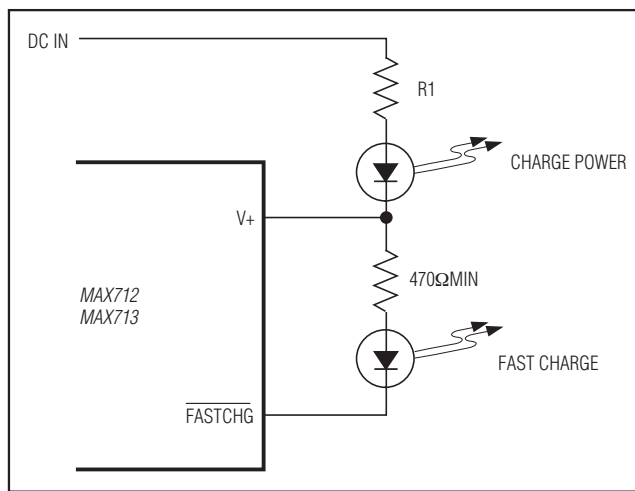
Figure 18. LED Connection for Status Outputs
