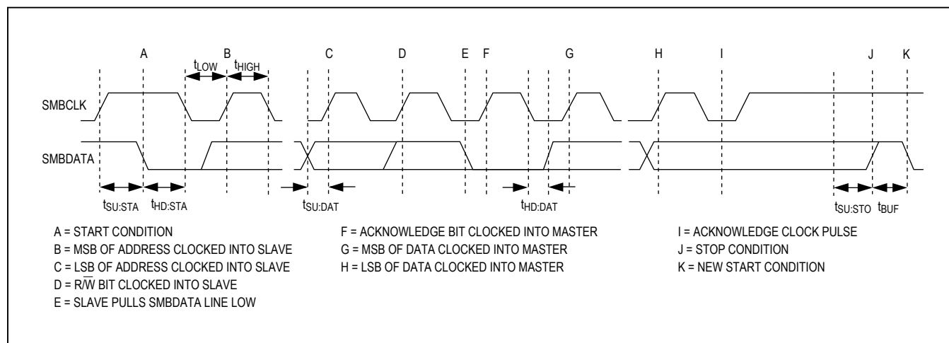
Figure 4. Read-Timing Diagram
