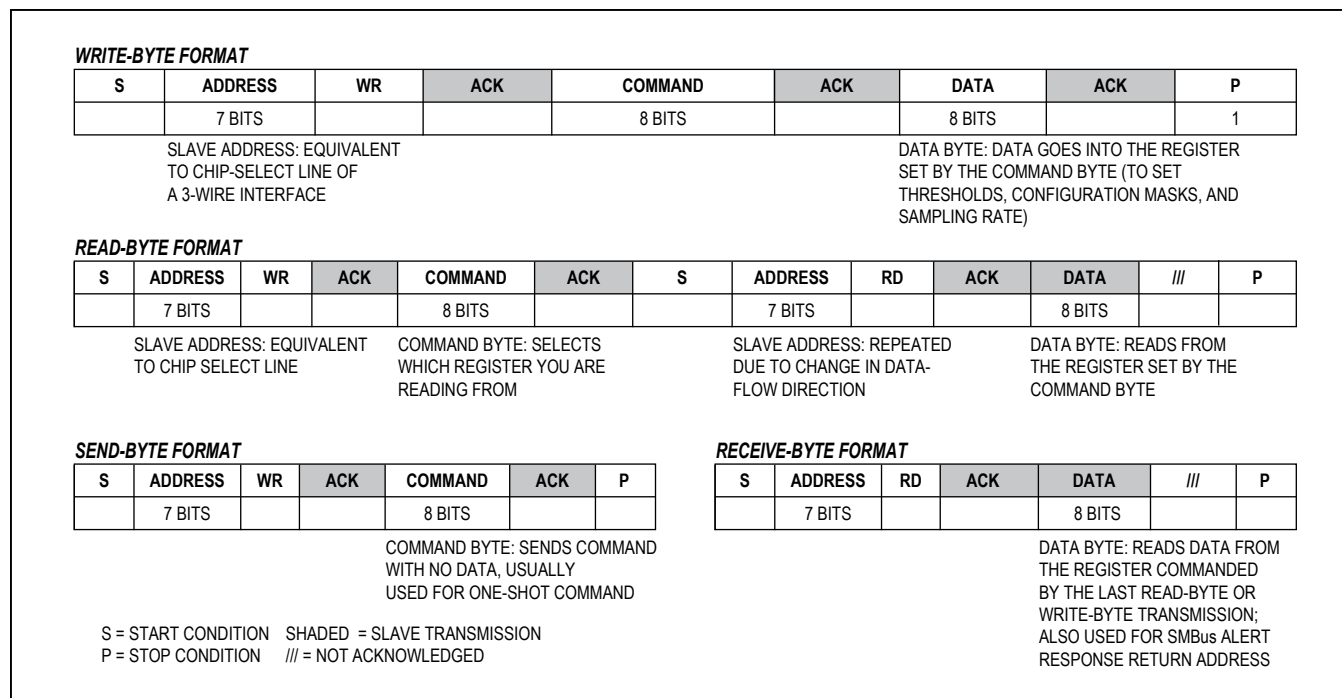
Figure 2. SMBus Protocols
