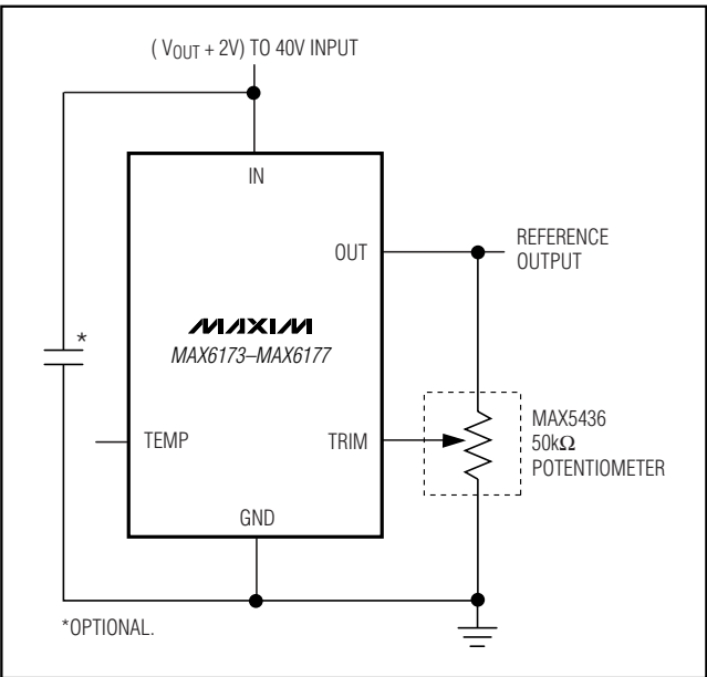
Figure 2. Applications Circuit Using the MAX5436 Potrntiometer
