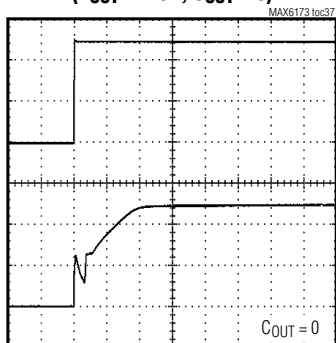
TURN-ON TRANSIENT ( V_{OUT} = 2.5V , C_{OUT} = 0 )
