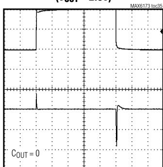
LINE TRANSIENT ( V_{OUT} = 2.5V )
