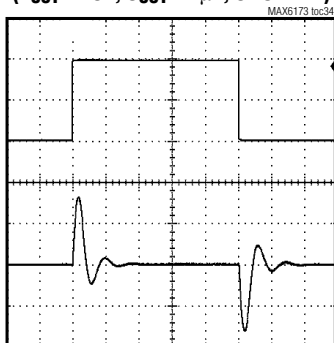
LOAD TRANSIENT ( V_{OUT} = 10V , C_{OUT} = 1\mu F , 0 TO -2mA)
