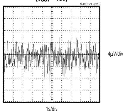
0.1Hz TO 10Hz OUTPUT NOISE ( V_{OUT} = 10V )
