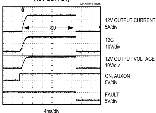
POWER-UP INTO FAULT (12V OUTPUT)
