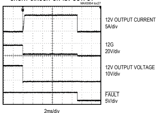
SHORT CIRCUIT ON 12V OUTPUT
