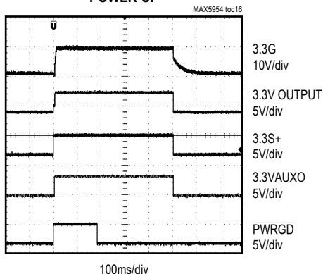
3.3V INPUT/3.3V AUXILIARY INPUT POWER-UP
