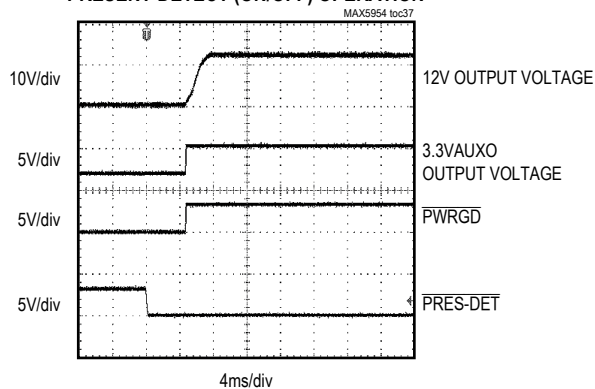
PRESENT-DETECT (ON/OFF) OPERATION
