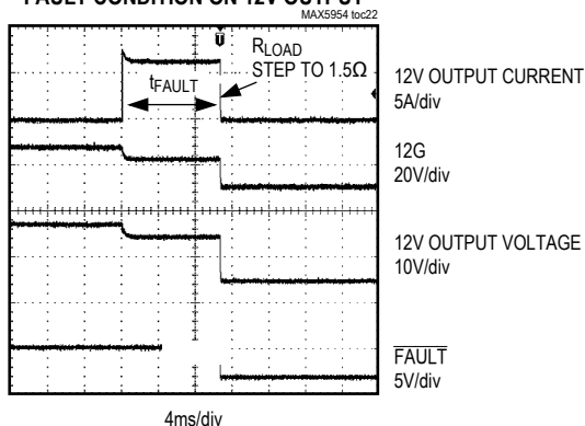
FAULT CONDITION ON 12V OUTPUT
