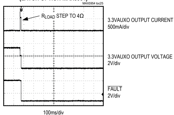
FAULT CONDITION ON AUXILIARY OUTPUT (LATCH OPTION MAX5954)
