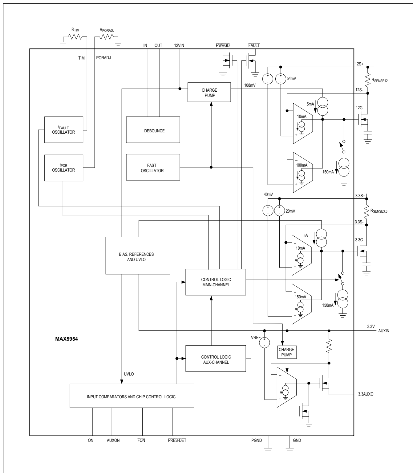
Figure 1. Functional Diagram
