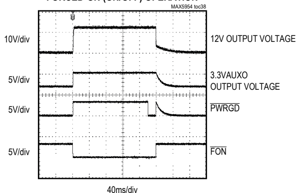
FORCED-ON (ON/OFF) OPERATION
