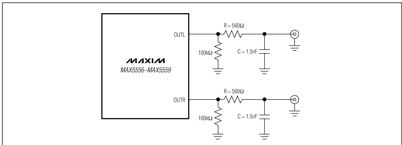
Figure 11. Passive Component Analog Output Filter
