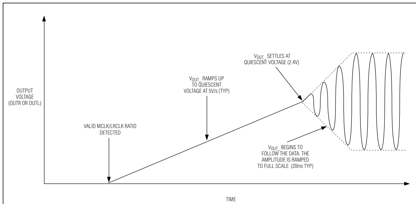
Figure 14. Power-Up Sequence
