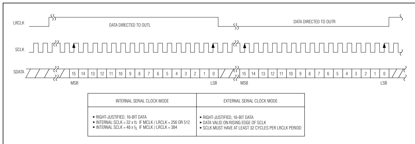
Figure 6. MAX5558 Data Format Timing
