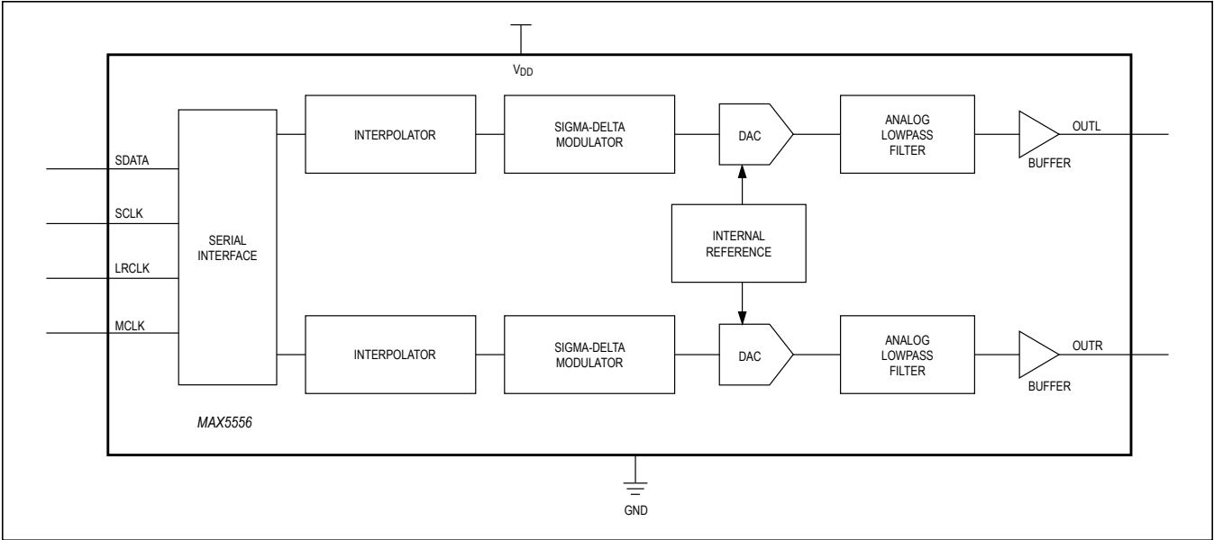
Figure 2. Functional Diagram
