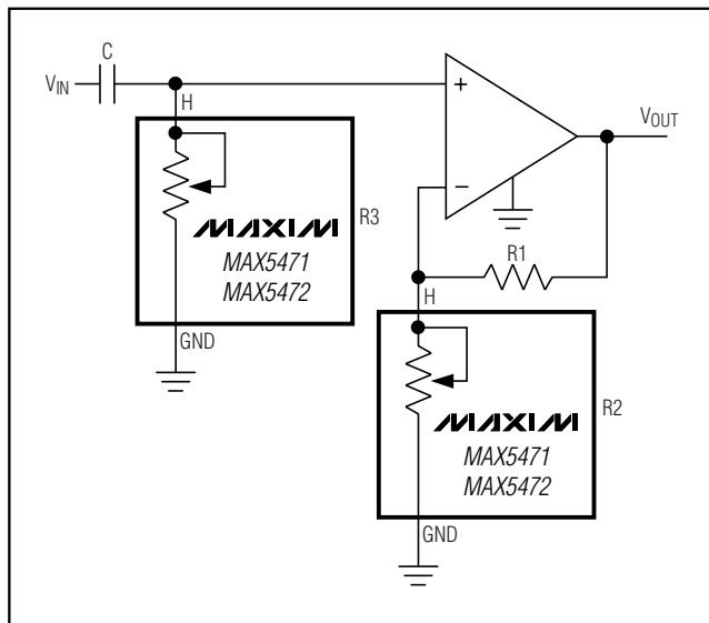
Figure 6. Programmable Filter
