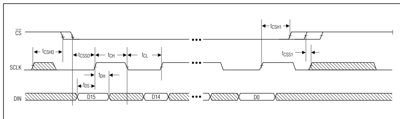
Figure 1. Timing Diagram
