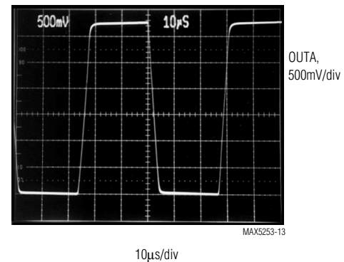
DYNAMIC RESPONSE
