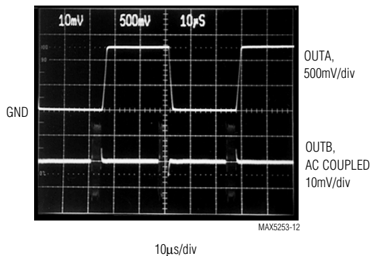
ANALOG CROSSTALK
