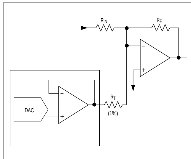
Figure 15a. Typical Trimming Circuit
