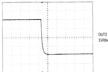
MAX520 NEGATIVE SETTLING TIME
