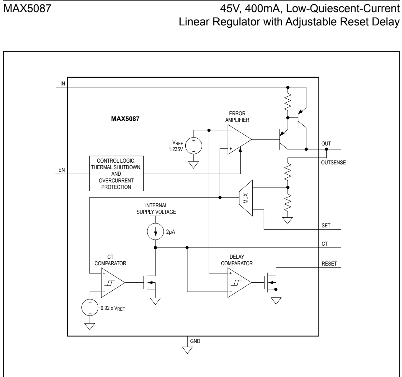
Figure 1. Functional Diagram
