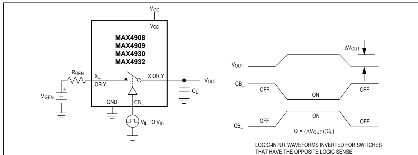
Figure 4. Charge Injection
