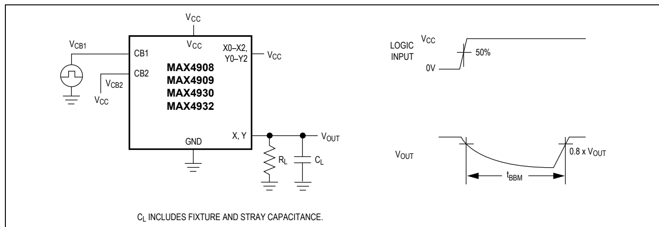
Figure 3. Break-Before-Make Interval
