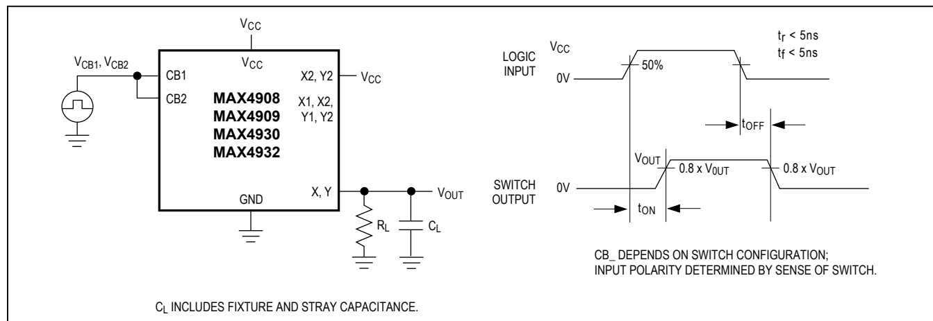
Figure 2. Switching Time
