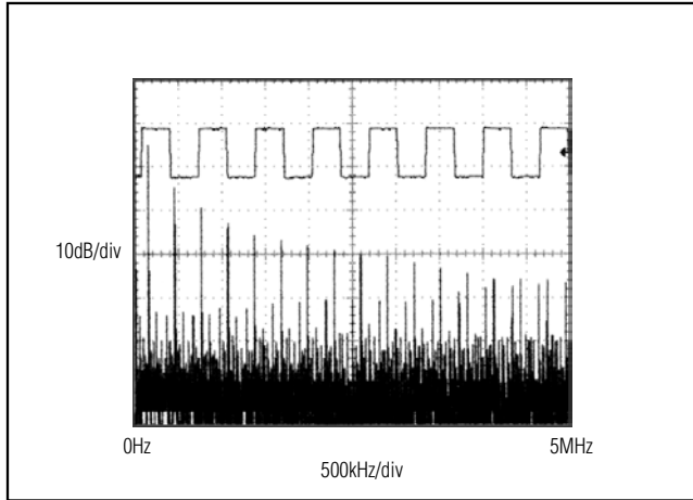
Figure 12. Driver Output Waveform and FFT Plot of MAX481/MAX483/MAX485/MAX487-MAX489 Transmitting a 150kHz Signal
