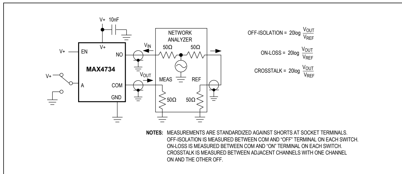
Figure 5. Off-Isolation/On-Channel/Crosstalk Bandwidth
