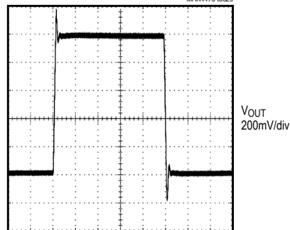
MAX4488/MAX4489 LARGE-SIGNAL PULSE RESPONSE
