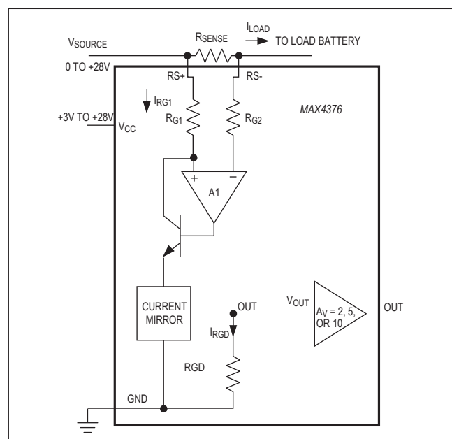
Figure 1. Functional Diagram
