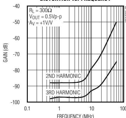
MAX4285/MAX4287/MAX4288 DISTORTION vs. FREQUENCY
