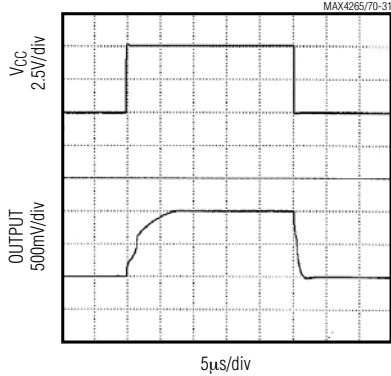
POWER-UP/POWER-DOWN RESPONSE
