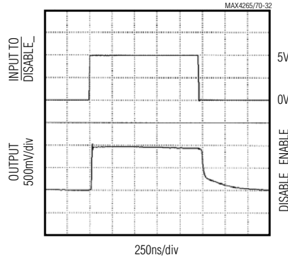
DISABLE/ENABLE RESPONSE
