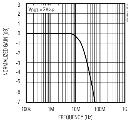
MAX4146 LARGE-SIGNAL vs. FREQUENCY ( A_V = +100 )
