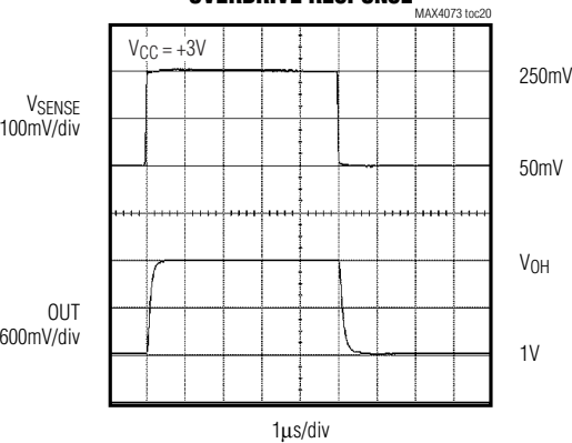
MAX4073T OVERDRIVE RESPONSE
