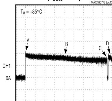
SHORT-CIRCUIT RESPONSE ( V_{\text{BIAS}} = 76\text{V} )
