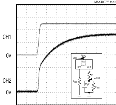
STARTUP DELAY ( V_{\text{BIAS}} = 5\text{V} , I_{\text{REF}} = 250\text{nA} )
