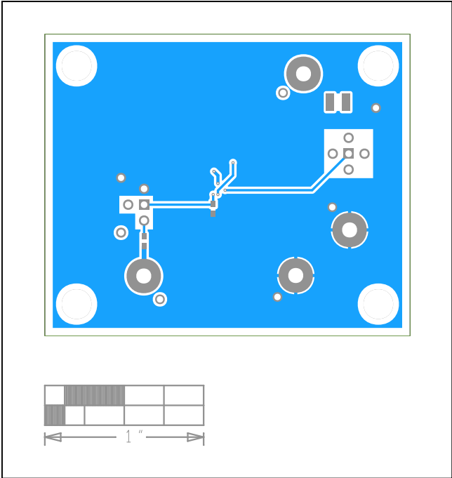
MAX38643A WLP EV Kit—Bottom
