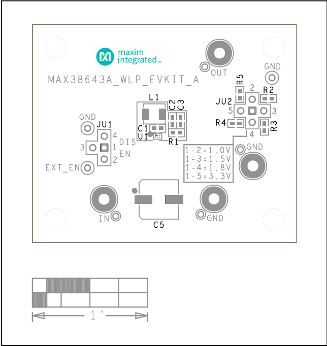
MAX38643A WLP EV Kit—Silk_Top
