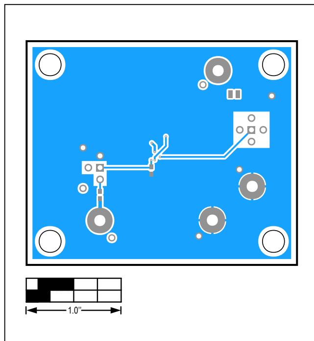
MAX38641A WLP EV Kit—Bottom View
