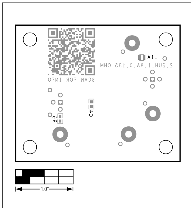
MAX38641A WLP EV Kit—Bottom Silkscreen
