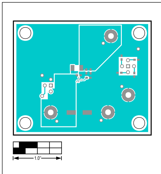
MAX38641A WLP EV Kit—Top View
