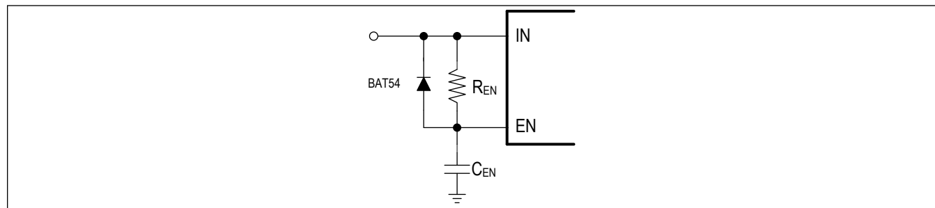
Figure 1. RC Circuit at EN
