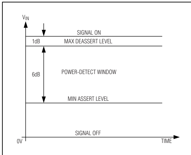
Figure 2. LOS Assert Threshold Set 1dB Below the Minimum by Receiver Sensitivity for Selected R_{TH}
