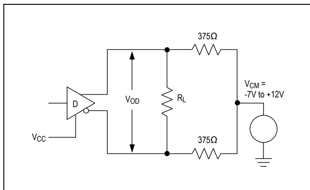
Figure 5. Driver V_{OD} with Varying Common-Mode Voltage
