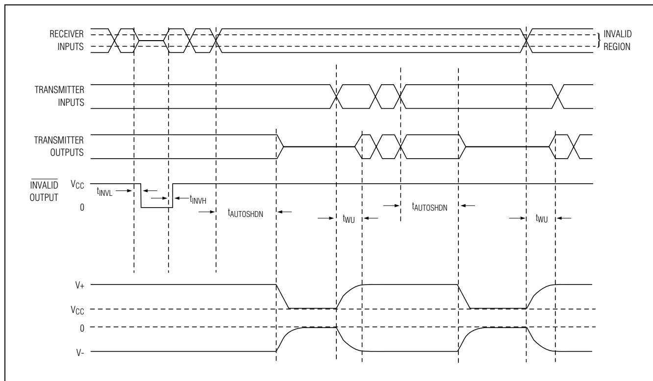
Figure 3b. AutoShutdown Plus/INVALID Timing Diagram
