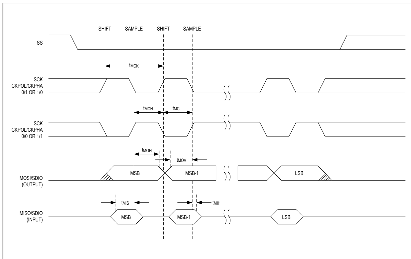
Figure 1. SPI Master/SPIX Master Communications Timing Diagram
