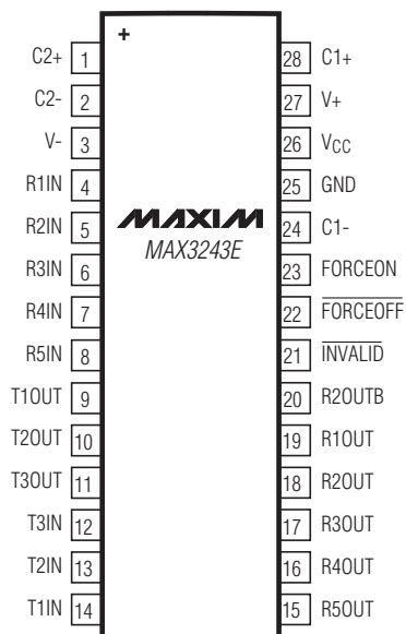
SO/SSOP/TSSOP
