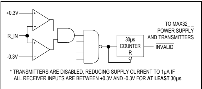
Figure 3a. MAX32__ Entering 1μA Supply Mode Through AutoShutdown
