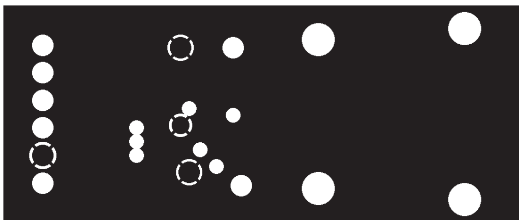
Figure 4. MAX31855PMB1 Peripheral Module PCB Layout—Inner Layer 1 (Ground)
