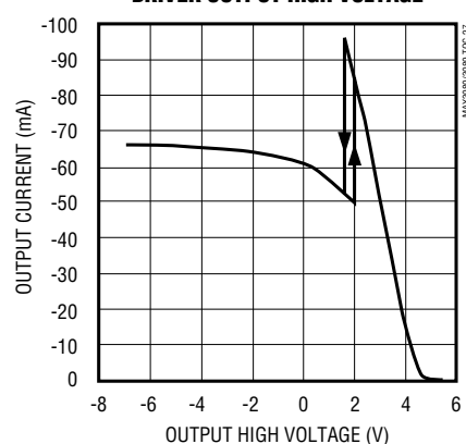
OUTPUT CURRENT vs. DRIVER OUTPUT HIGH VOLTAGE
