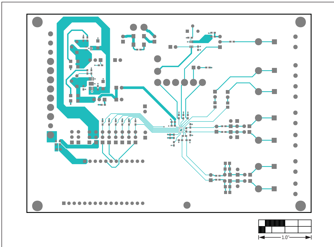
MAX30001 EV Kit—Top
