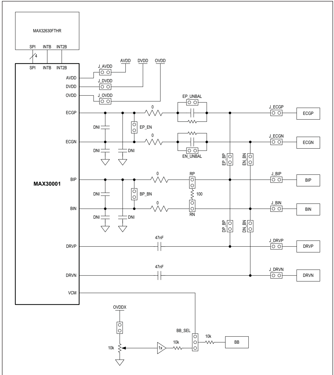
Figure 17. Simplified Schematic.
