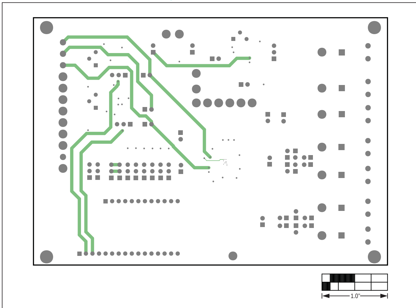
MAX30001 EV Kit—Layer 3
