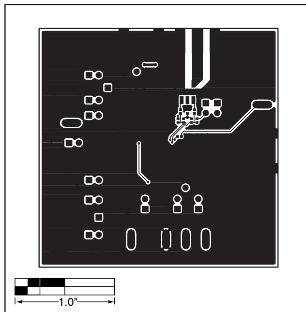
Figure 8. MAX2900-MAX2904 EV Kits PC Board Layout—Solder Side
