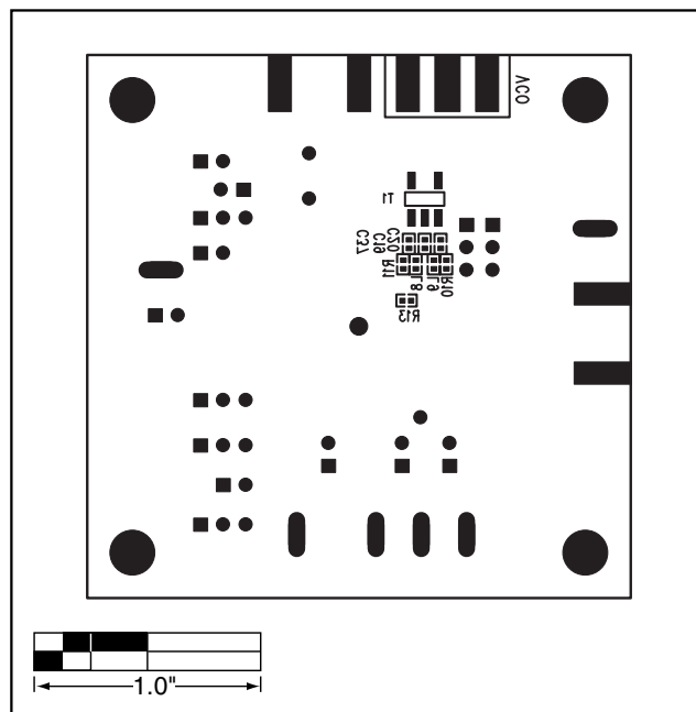
Figure 6. MAX2900-MAX2904 EV Kits—Bottom Silkscreen
