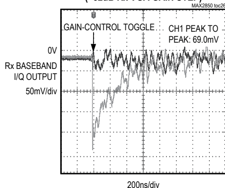
Rx DC OFFSET SETTLING RESPONSE (+32dB Rx VGA GAIN STEP)
