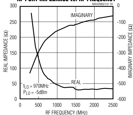
MAX2680 RF PORT IMPEDANCE vs. RF FREQUENCY
