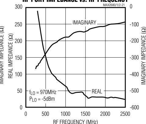
MAX2682 RF PORT IMPEDANCE vs. RF FREQUENCY
