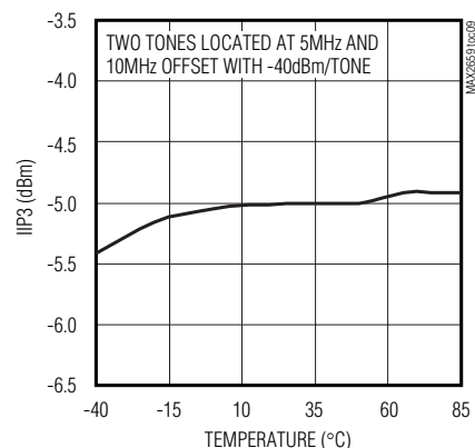
IIP3 vs. TEMPERATURE
