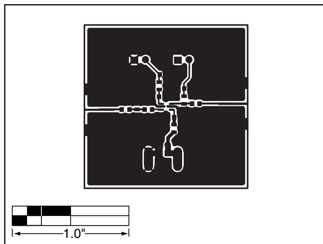
Figure 3. MAX2642/MAX2643 EV Kits PC Board Layout—Component Side
