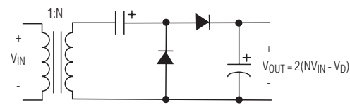
FIGURE 1B. VOLTAGE DOUBLER
