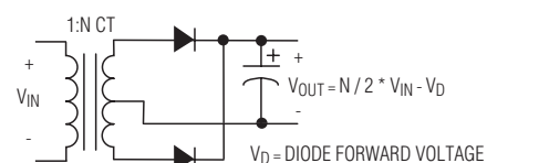
FIGURE 1A. PUSH-PULL RECTIFICATION
