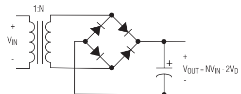
FIGURE 1C. FULL-WAVE RECTIFIER
