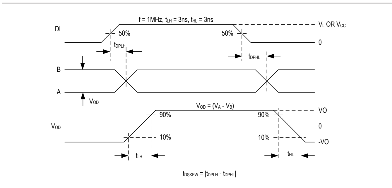
Figure 4: Driver Propagation Delays
