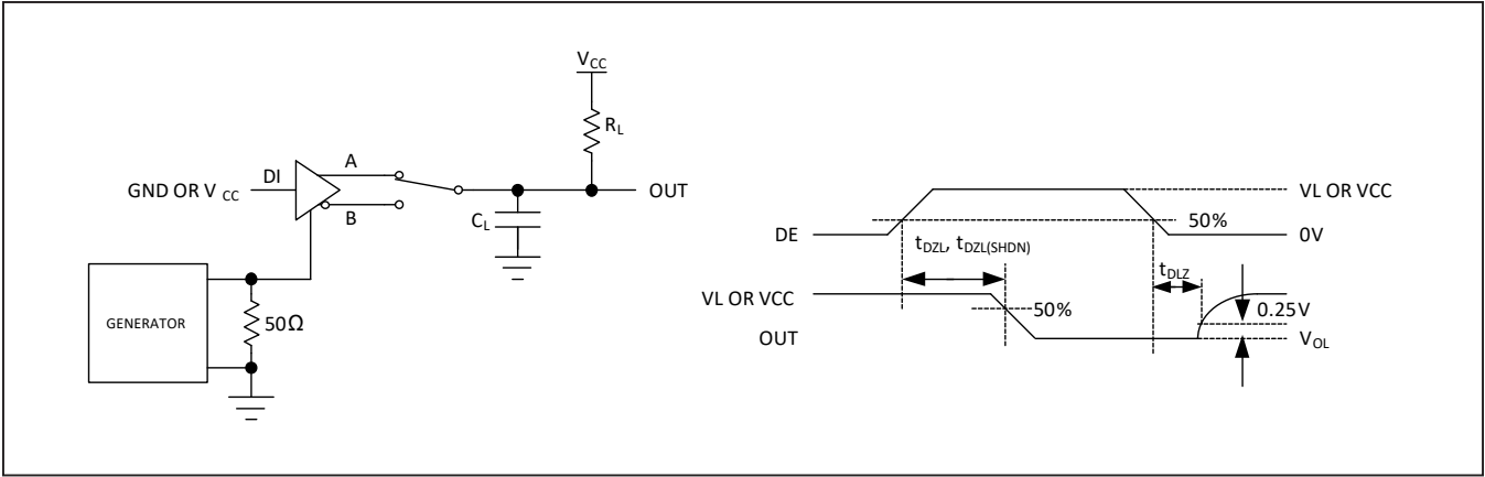
Figure 6: Driver Enable and Disable Times ( t_{DZL} , t_{DLZ} )
