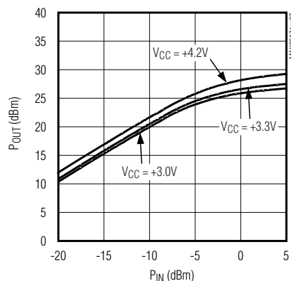
OUTPUT POWER vs. INPUT POWER
