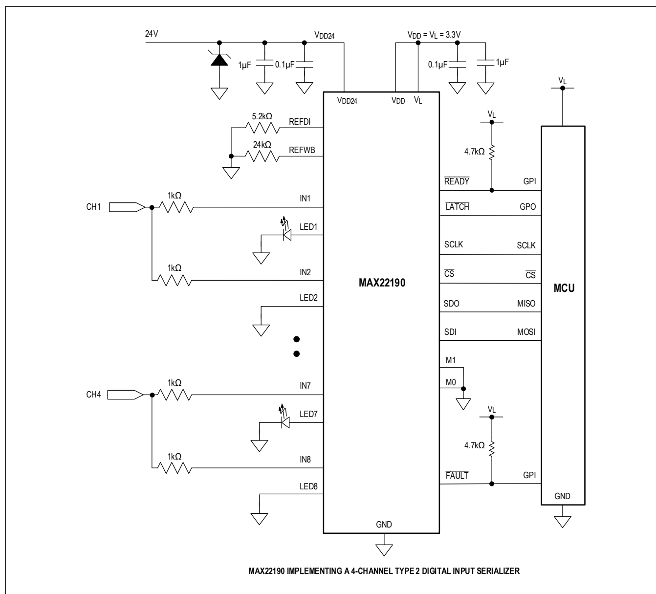
Figure 11. Implementing Type 2 Digital Inputs with MAX22190
