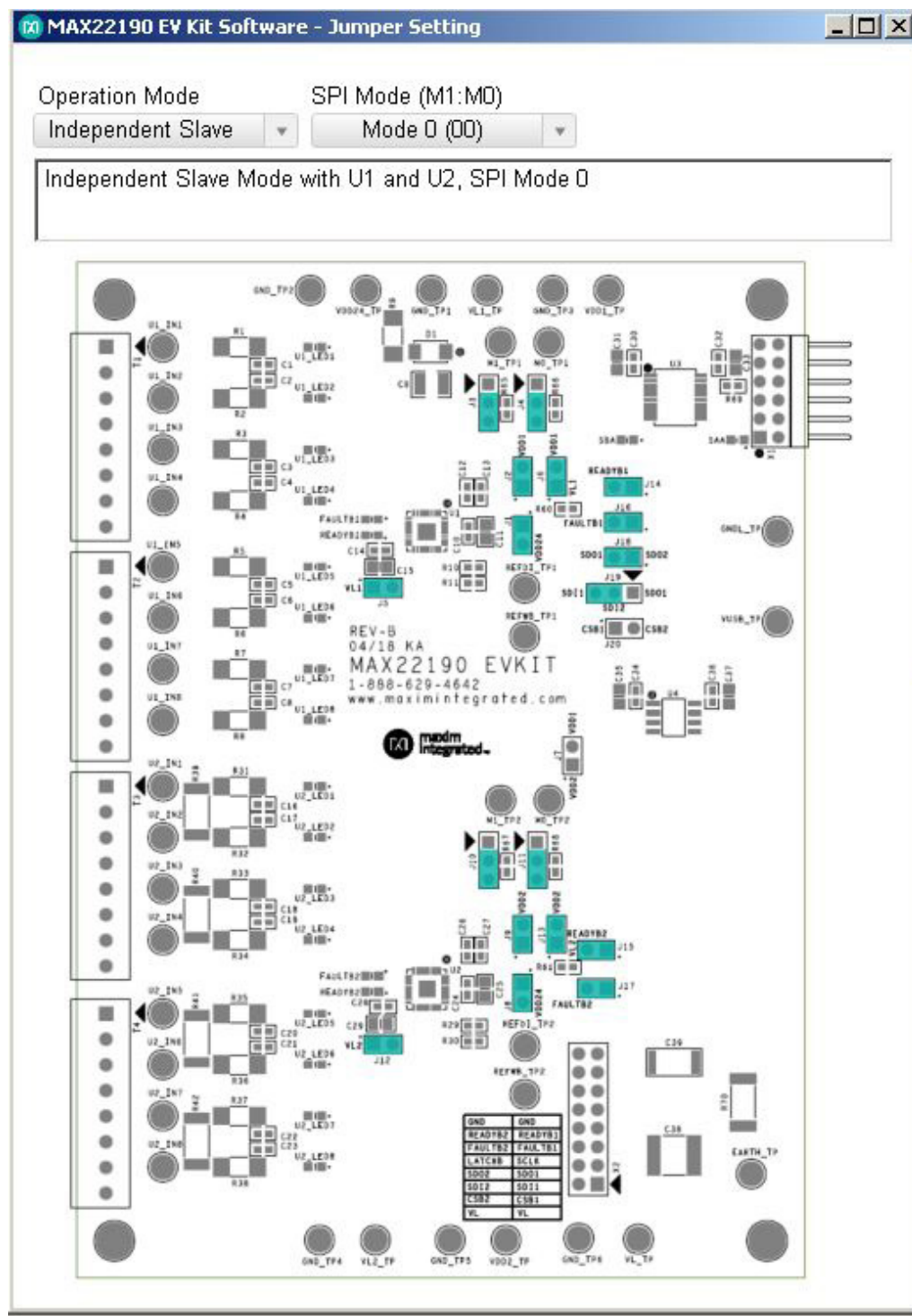
Figure 7. MAX22190 EV Kit Software—Jumper Setting Diagram
