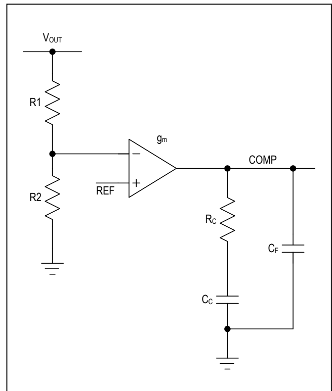
Figure 3. Compensation Network
