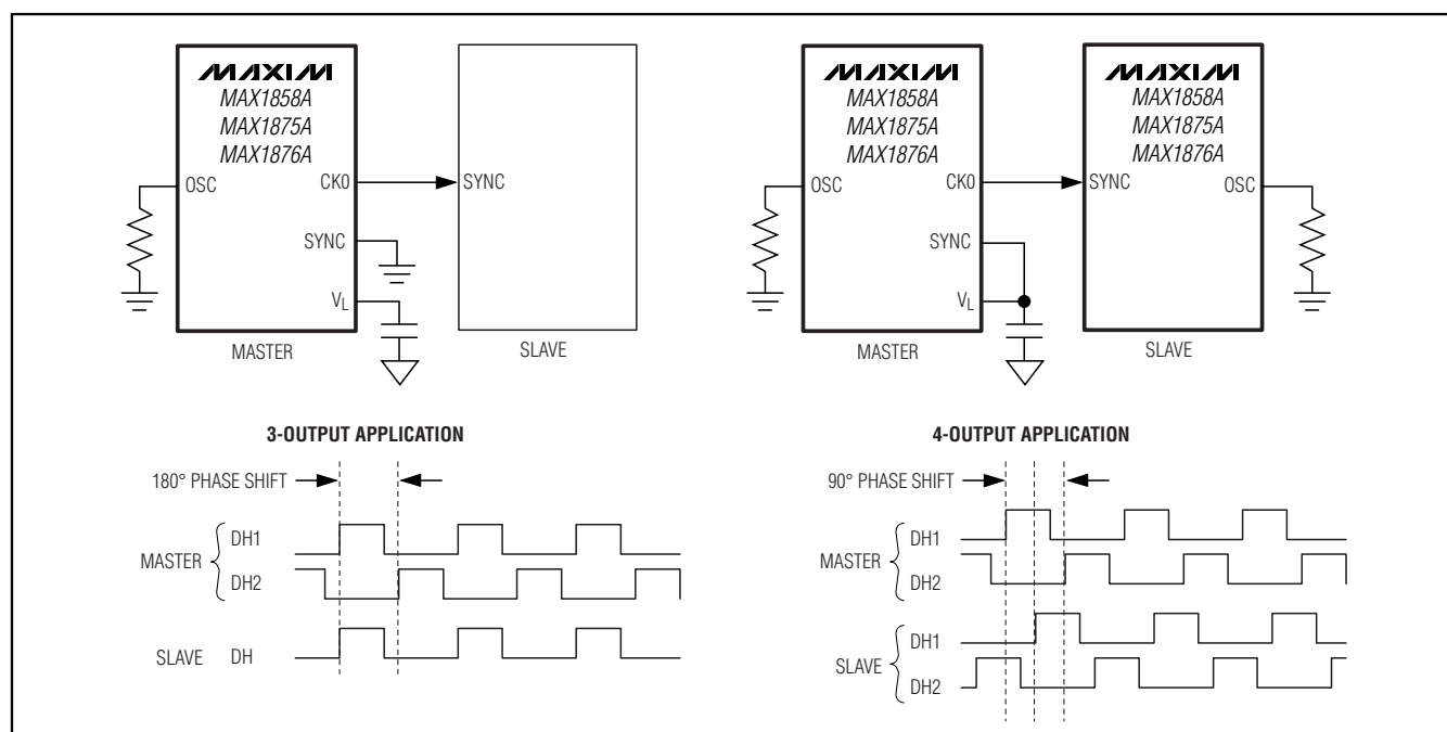
Figure 7. Synchronized Controllers
