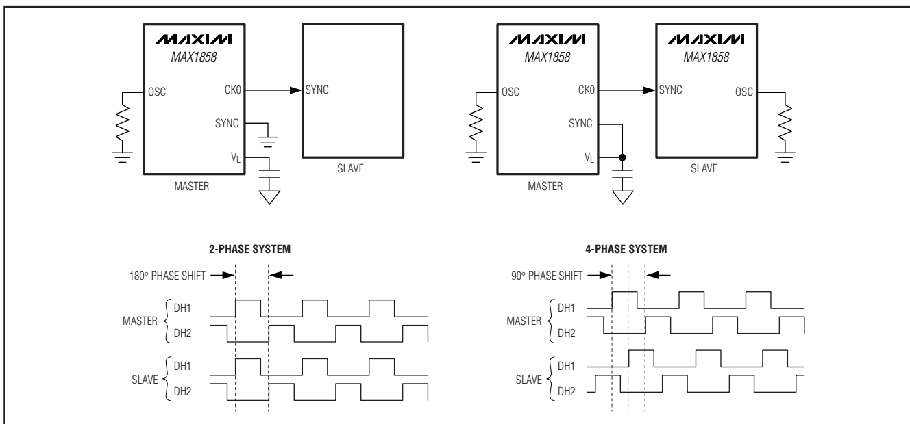
Figure 5. Synchronized Controllers
