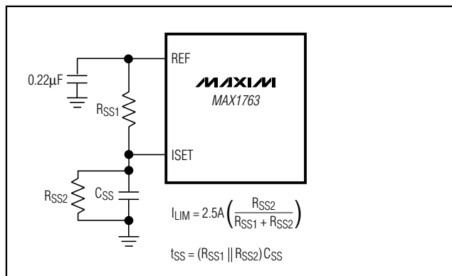
Figure 8. Soft-Start with Reduced Switch Limit Current
