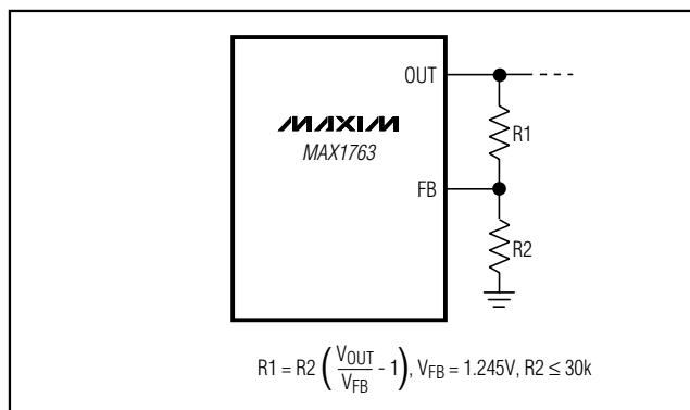
Figure 6. Connecting Resistors for External Feedback
