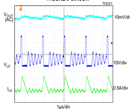
STEADY-STATE SWITCHING WAVEFORMS, 5V OUTPUT, DCM MODE, 25mA LOAD CURRENT, FIGURE 3 CIRCUIT
