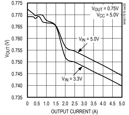
LOAD REGULATION ( V_{OUT} = 0.75V )
