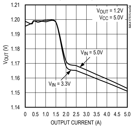
LOAD REGULATION ( V_{OUT} = 1.2V )
