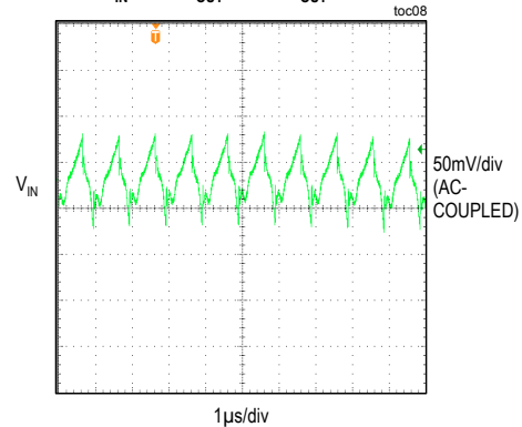
INPUT VOLTAGE RIPPLE V_{IN} = 5V , V_{OUT} = 1.2V , I_{OUT} = 5A
