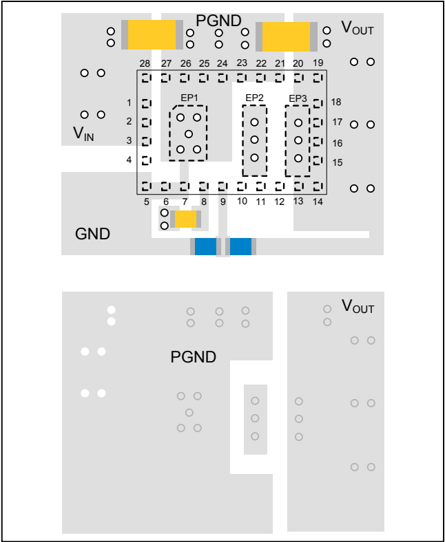
Figure 2. Layout Recommendation
