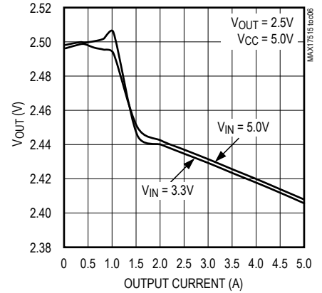
LOAD REGULATION ( V_{OUT} = 2.5V )
