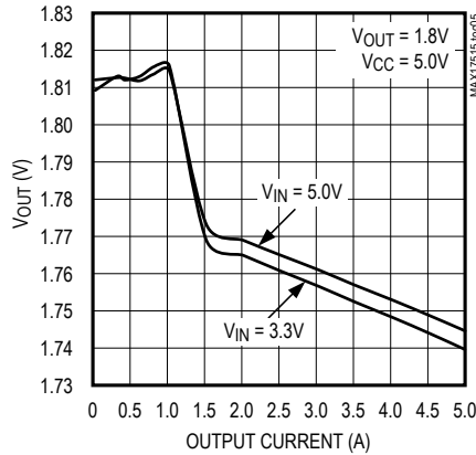
LOAD REGULATION ( V_{OUT} = 1.8V )
