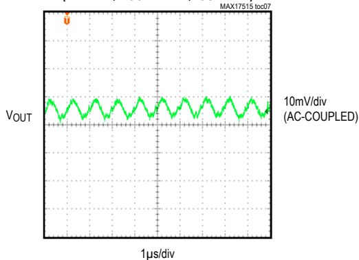
OUTPUT-VOLTAGE RIPPLE ( V_{IN} = 5V , V_{OUT} = 1.2V , I_{OUT} = 5A )
